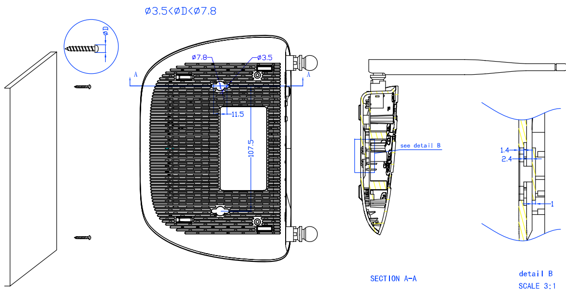
Figure 2-3 Wall-mount Install
