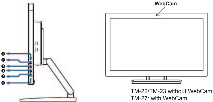
Figure 4 External Control Button
