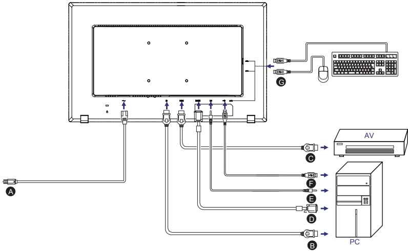
Figure 3 Connecting Cables
